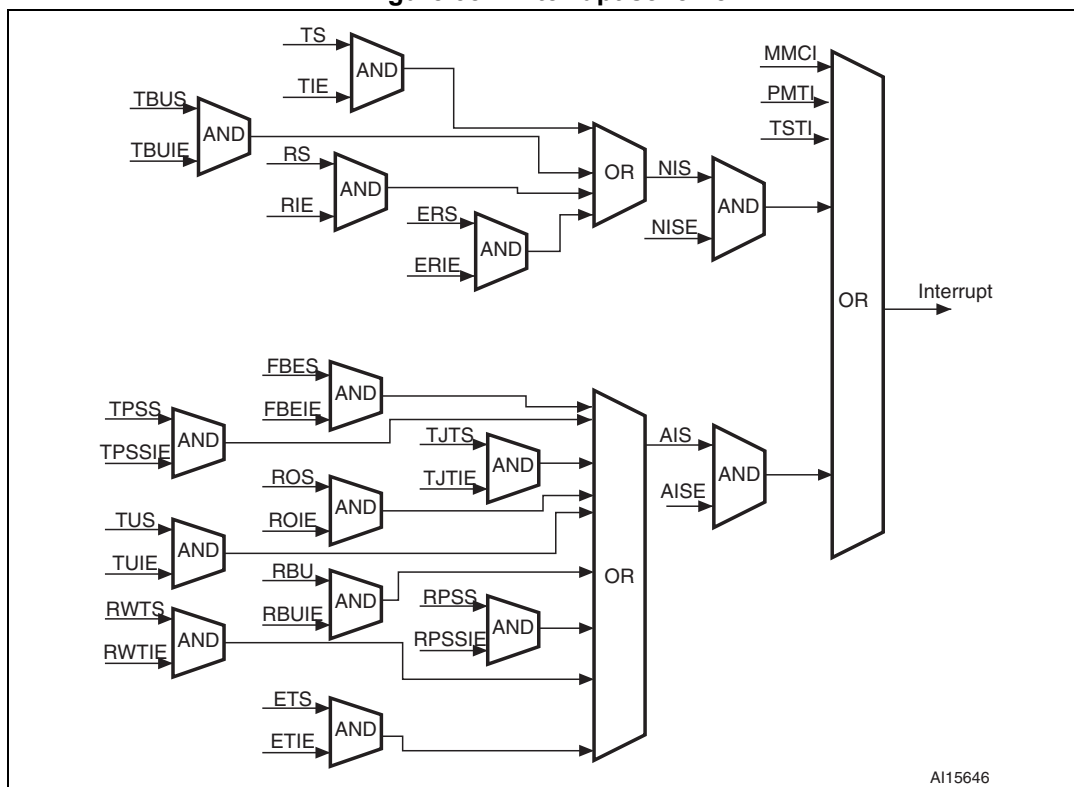
Figure 384. Interrupt scheme
