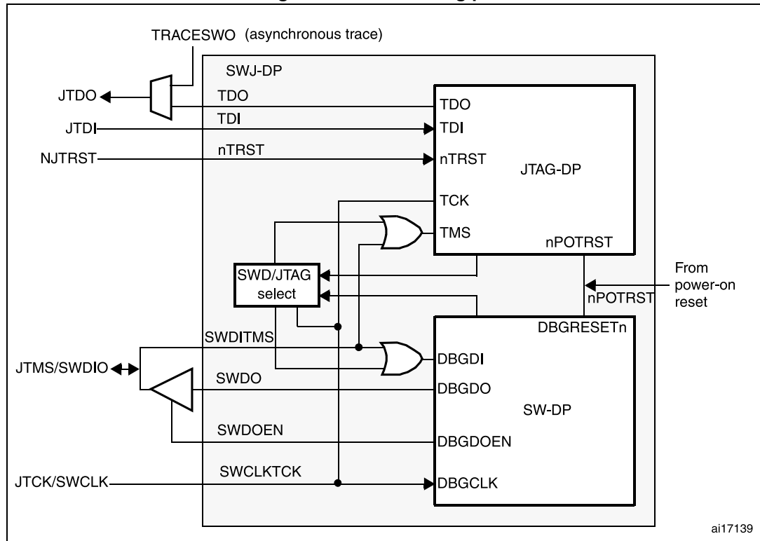
Figure 484. SWJ debug port
