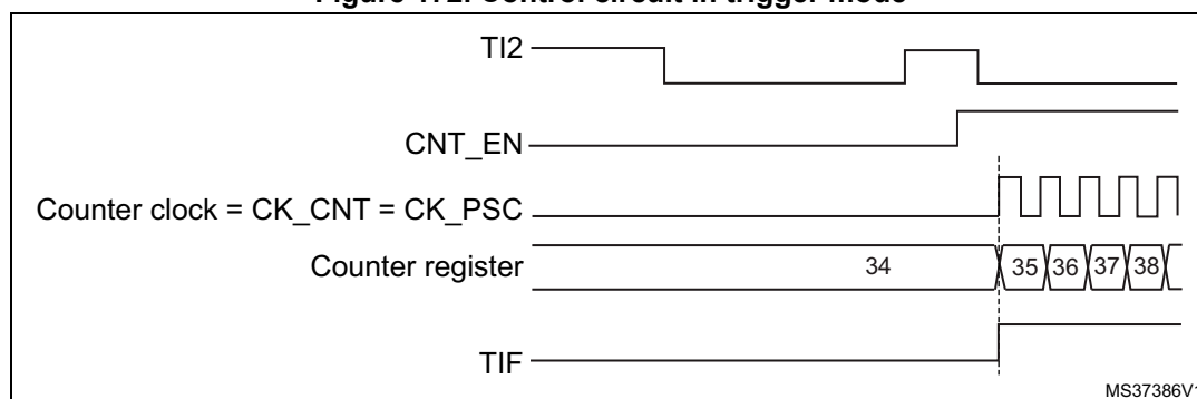
Figure 172. Control circuit in trigger mode
