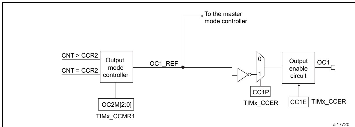
Figure 195. Output stage of capture/compare channel (channel 1)
