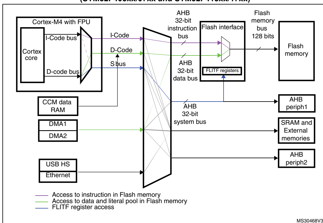
Figure 3. Flash memory interface connection inside system architecture (STM32F405xx/07xx and STM32F415xx/17xx)
