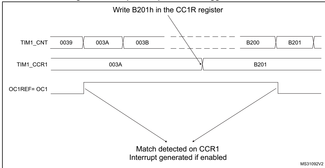
Figure 117. Output compare mode, toggle on OC1.
