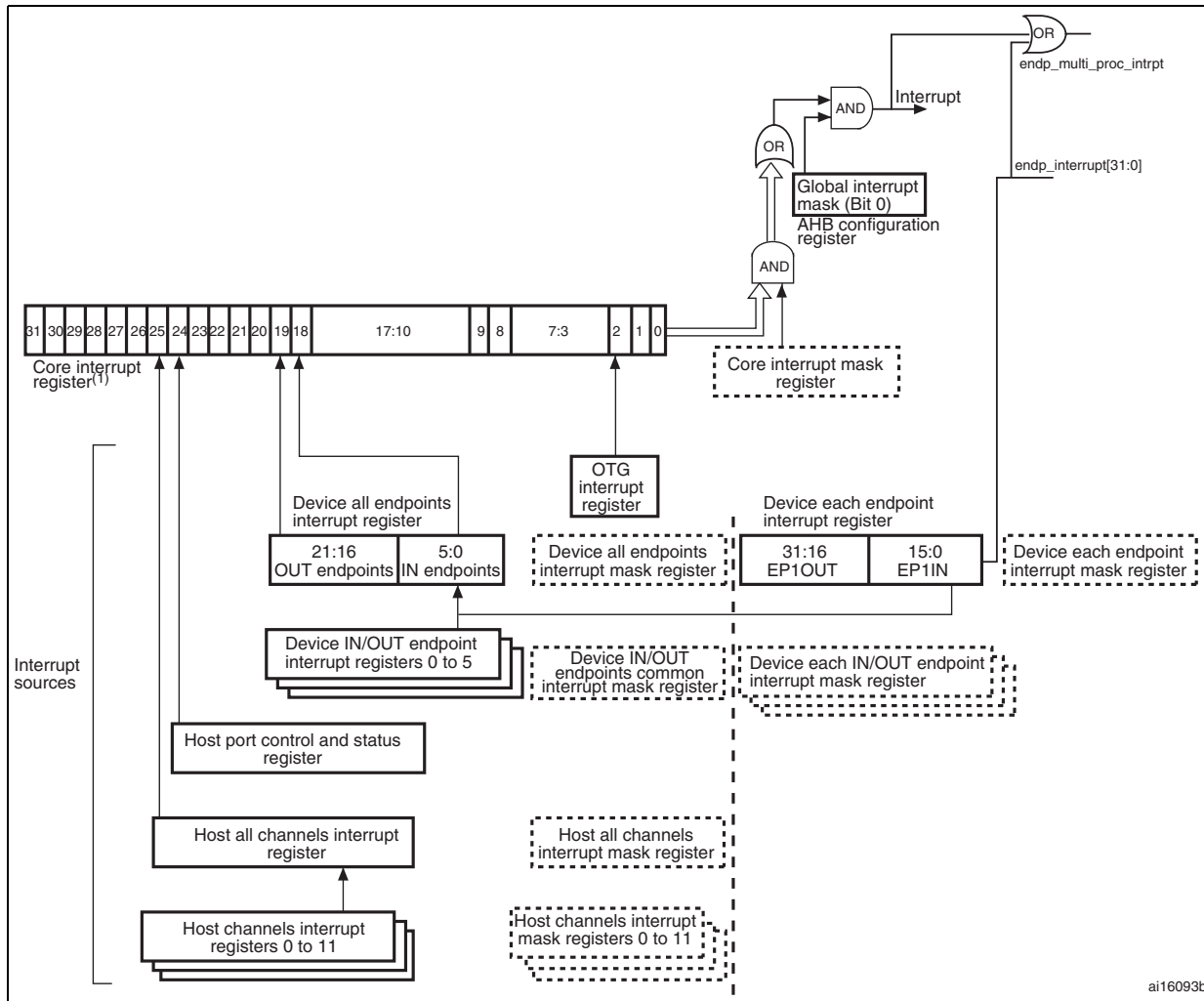
Figure 412. Interrupt hierarchy
