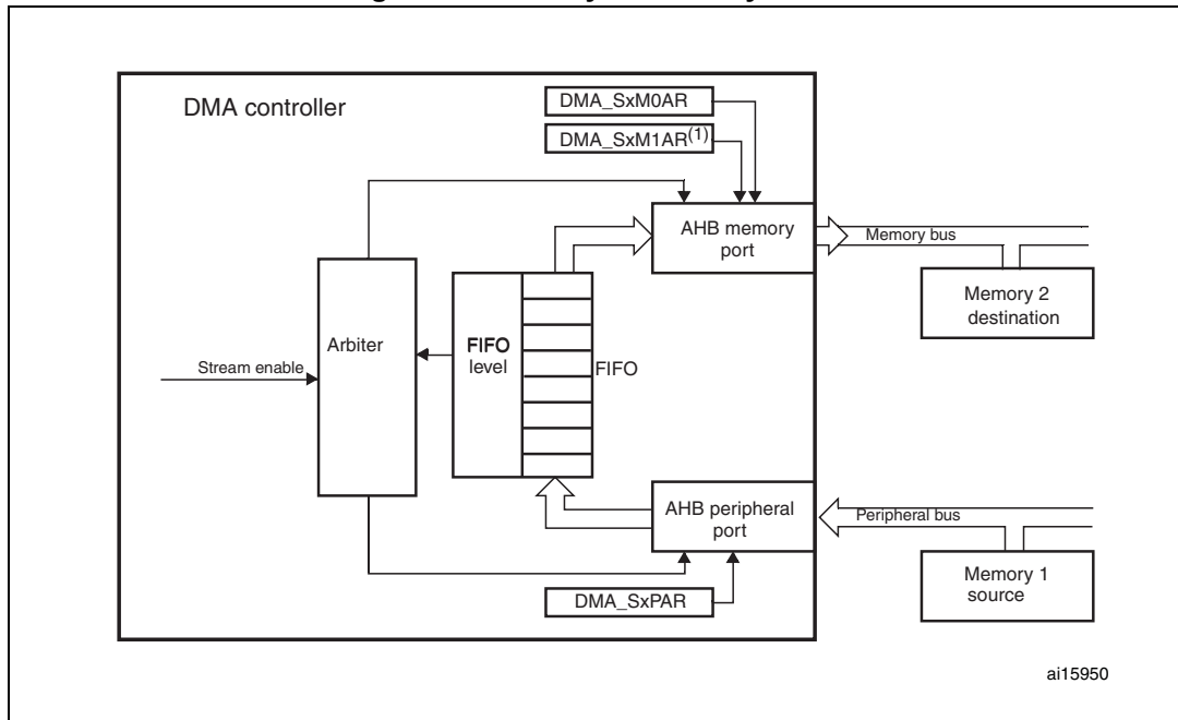
Figure 38. Memory-to-memory mode
