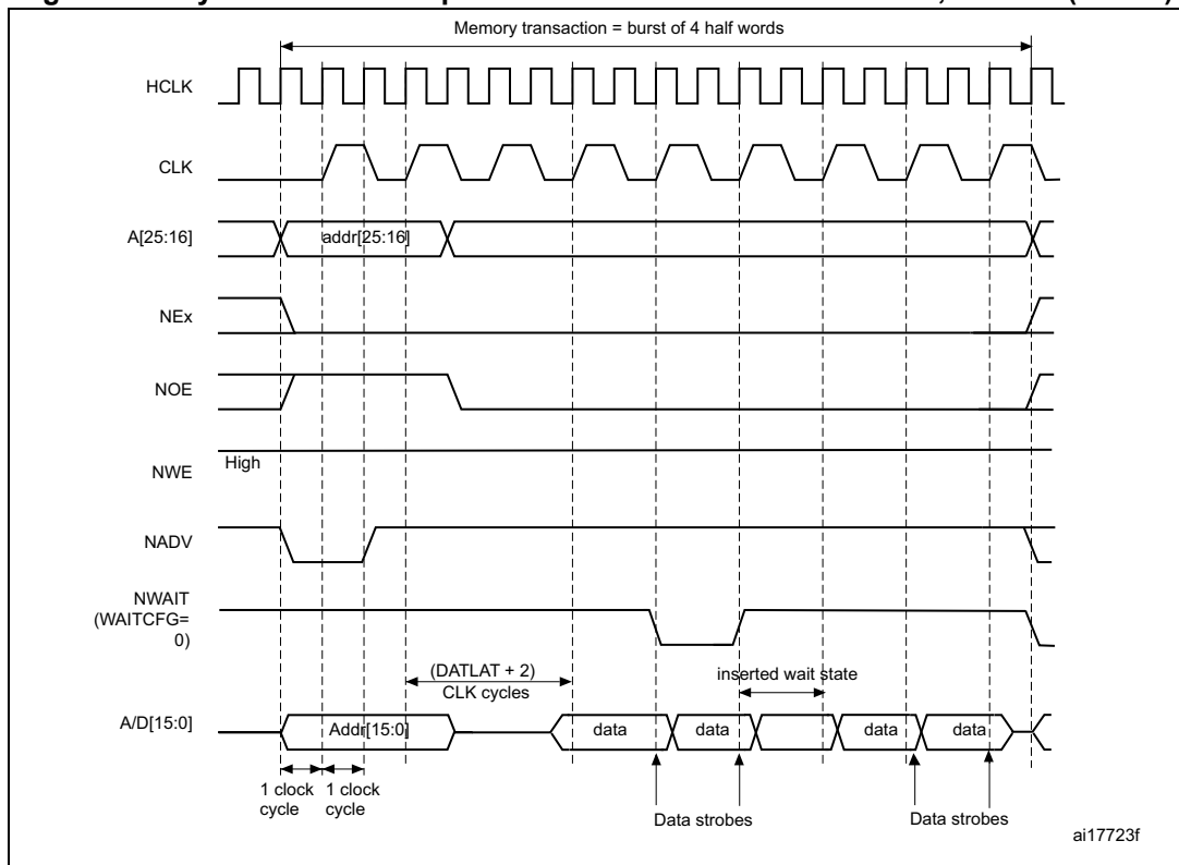
Figure 472. Synchronous multiplexed read mode waveforms - NOR, PSRAM (CRAM)
