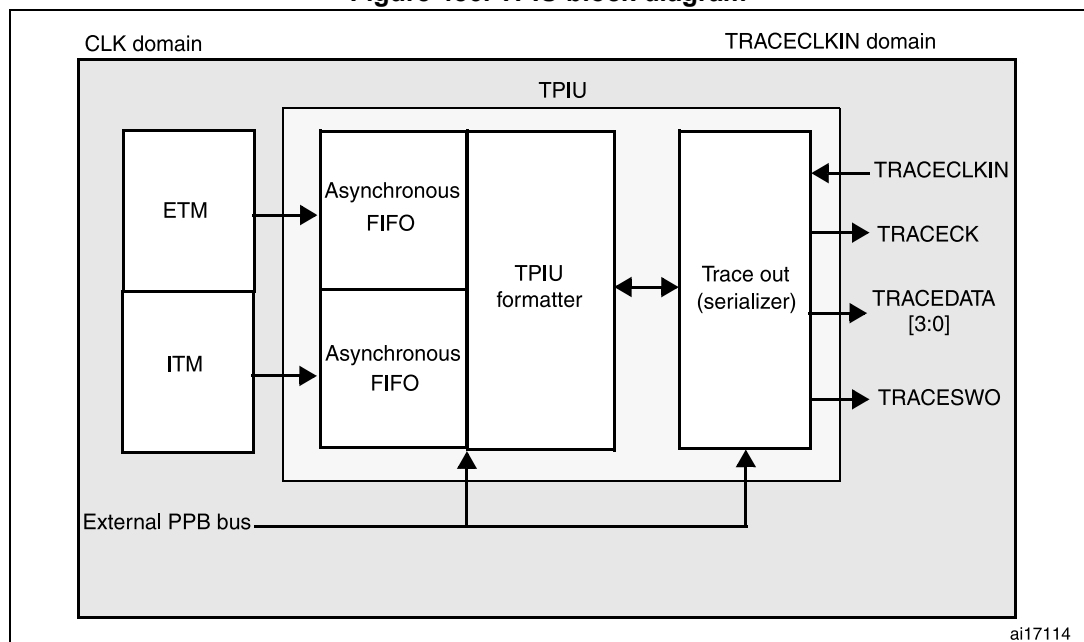
Figure 486. TPIU block diagram
