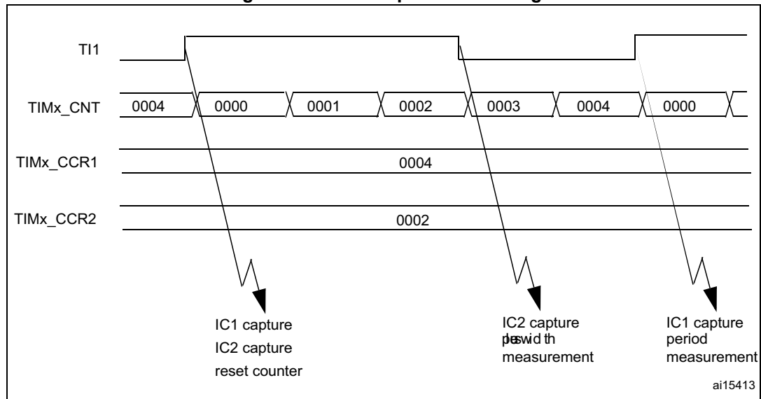
Figure 162. PWM input mode timing
