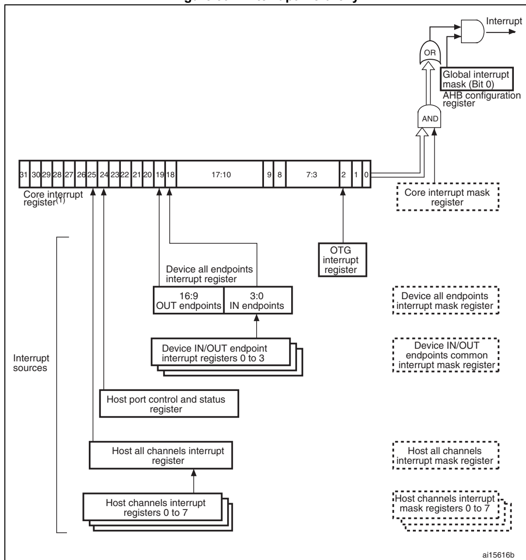
Figure 394. Interrupt hierarchy
