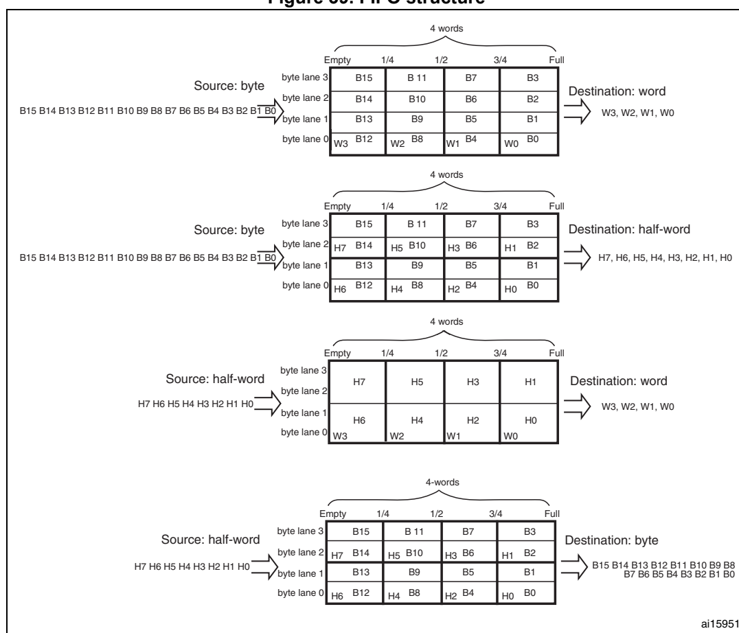
Figure 39. FIFO structure
