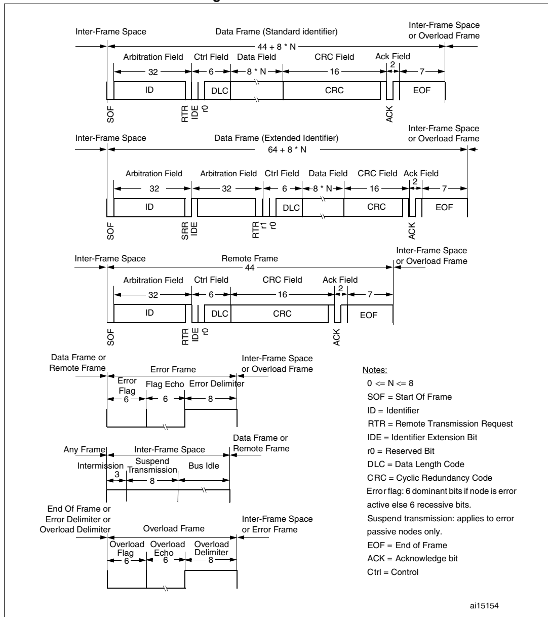
Figure 347. CAN frames
