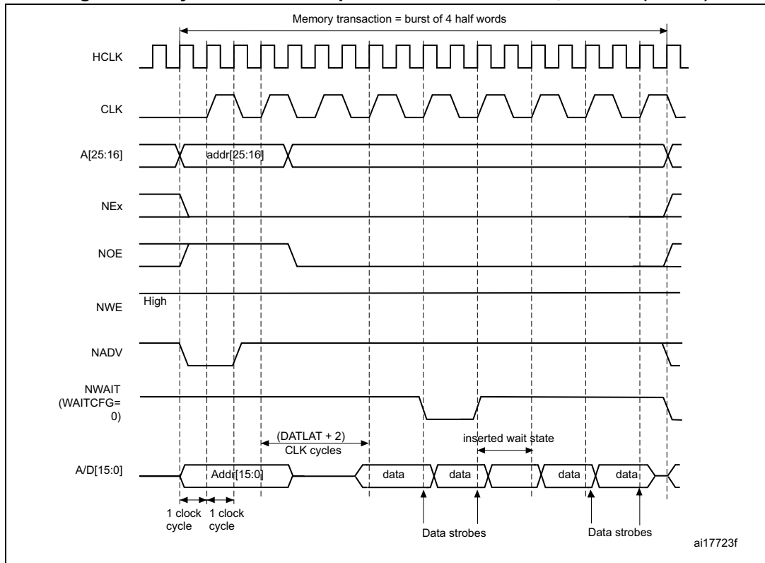
Figure 450. Synchronous multiplexed read mode - NOR, PSRAM (CRAM)
