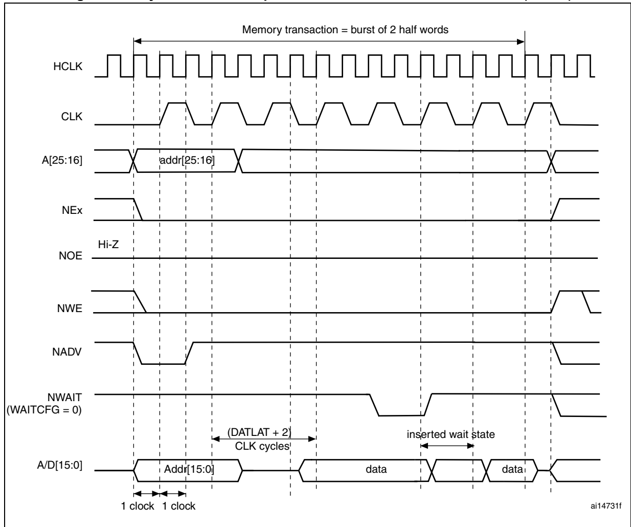
Figure 473. Synchronous multiplexed write mode waveforms - PSRAM (CRAM)
